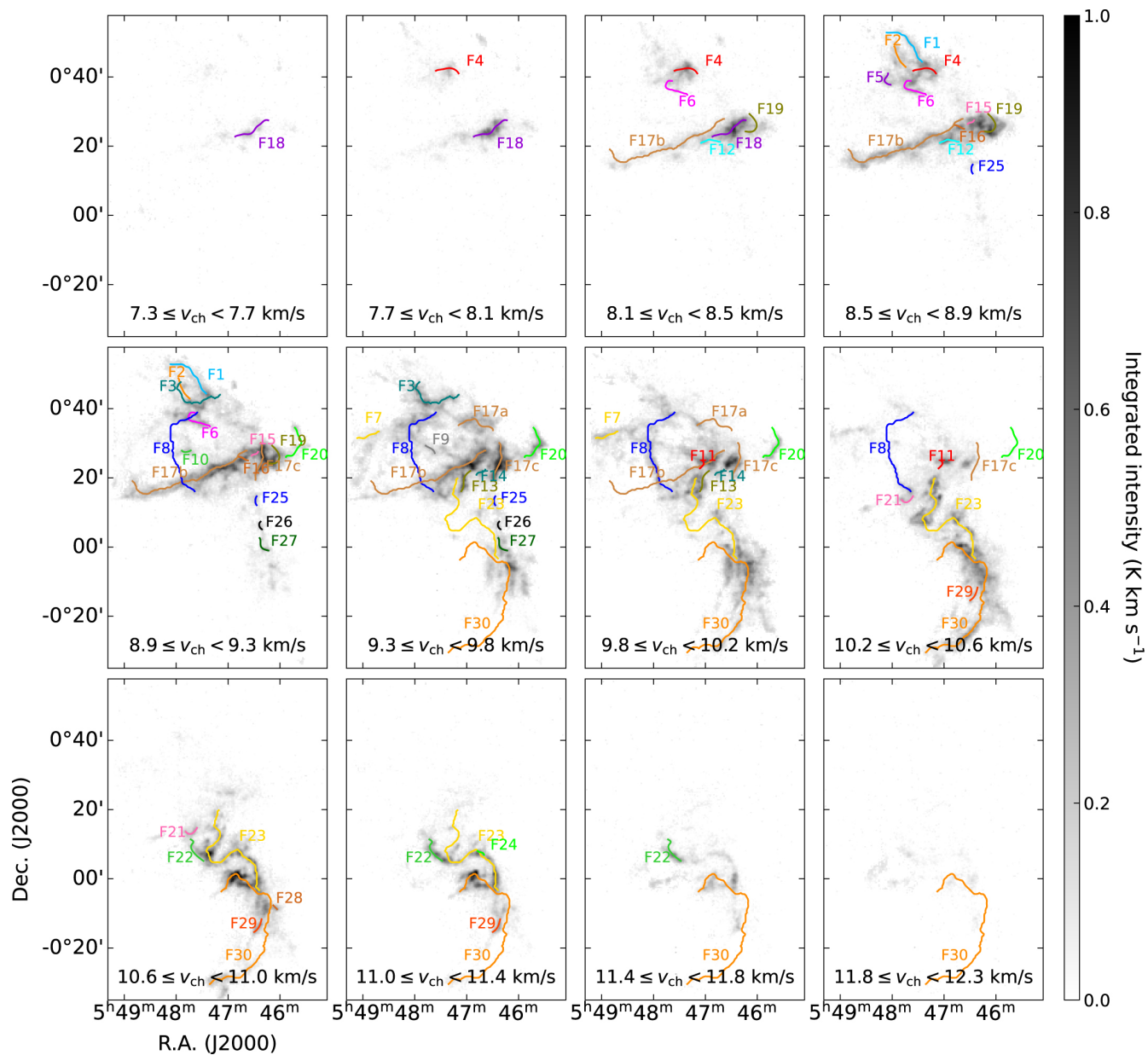
Figure 8. from Hyunju Yoo et al 2023 Astrophys. J. 957 doi:10.3847/1538-4357/acf8c2 https://dx.doi.org/10.3847/1538-4357/acf8c2 © 2023. The Author(s). Published by the American Astronomical Society.
