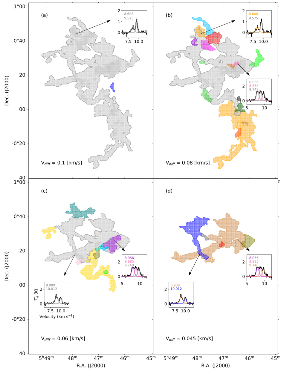
Figure 6. from Hyunju Yoo et al 2023 Astrophys. J. 957 doi:10.3847/1538-4357/acf8c2 https://dx.doi.org/10.3847/1538-4357/acf8c2 © 2023. The Author(s). Published by the American Astronomical Society.
