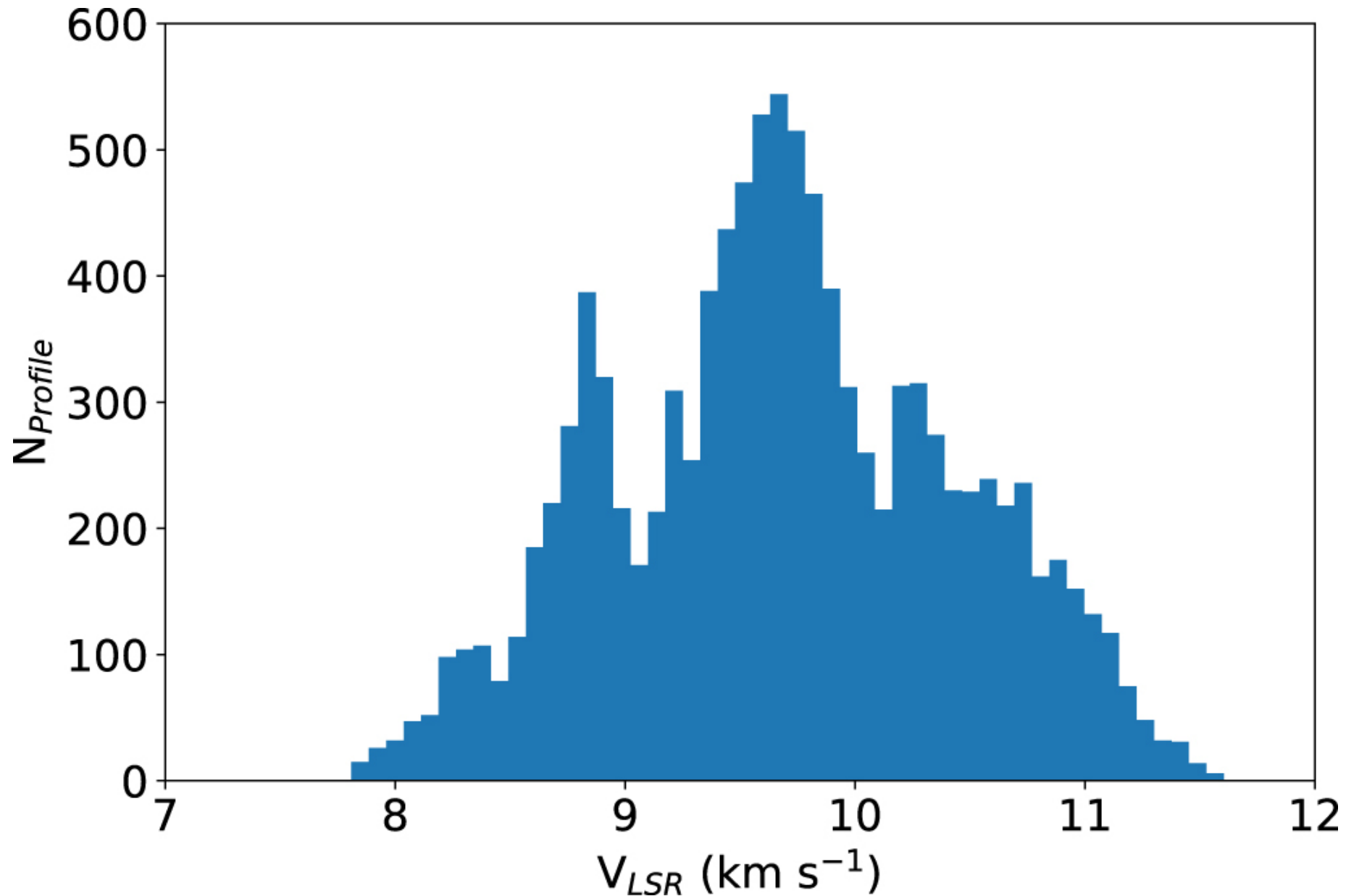
Figure 5. from Hyunju Yoo et al 2023 Astrophys. J. 957 doi:10.3847/1538-4357/acf8c2 https://dx.doi.org/10.3847/1538-4357/acf8c2 © 2023. The Author(s). Published by the American Astronomical Society.
