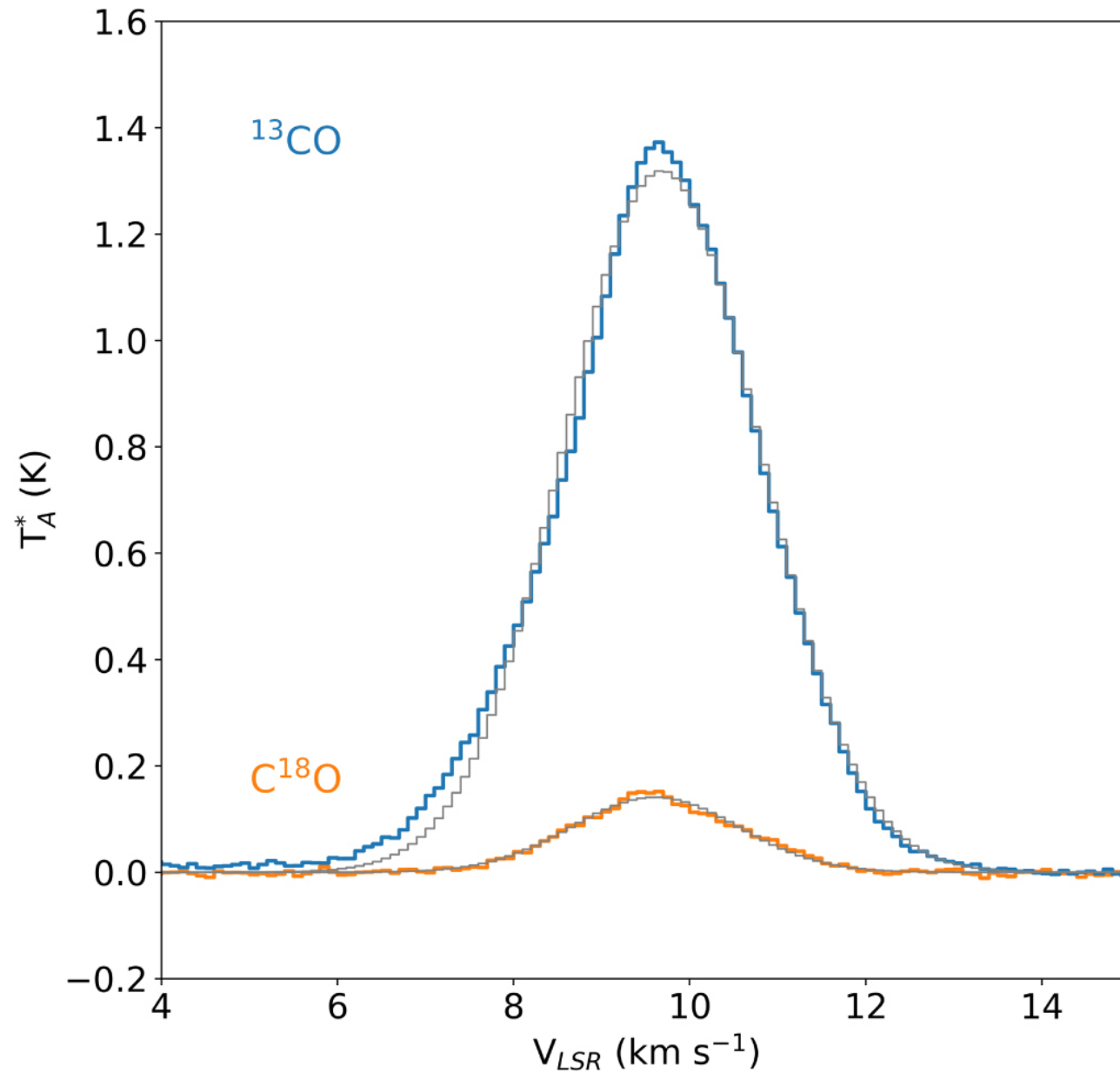
Figure 4. from Hyunju Yoo et al 2023 Astrophys. J. 957 doi:10.3847/1538-4357/acf8c2 https://dx.doi.org/10.3847/1538-4357/acf8c2 © 2023. The Author(s). Published by the American Astronomical Society.
