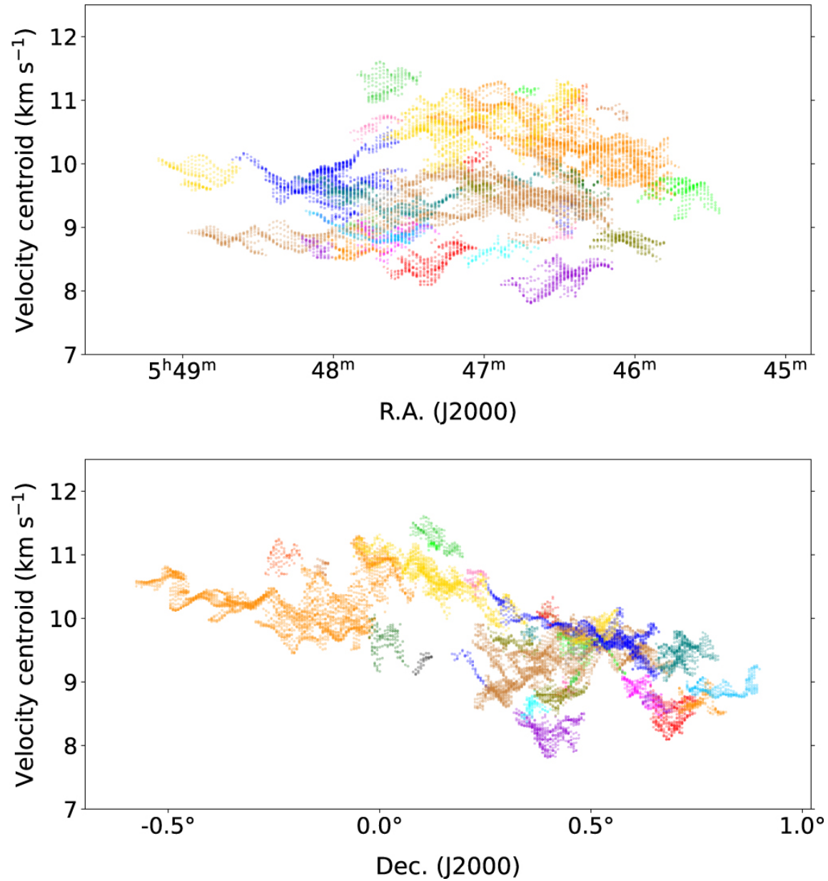
Figure 10. from Hyunju Yoo et al 2023 Astrophys. J. 957 doi:10.3847/1538-4357/acf8c2 https://dx.doi.org/10.3847/1538-4357/acf8c2 © 2023. The Author(s). Published by the American Astronomical Society.
