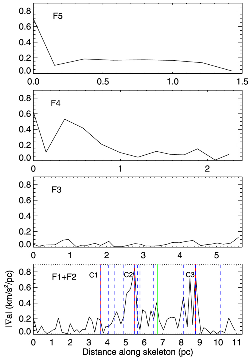
Figure 8. from Yu-Xin He et al 2023 Astrophys. J. 957 doi:10.3847/1538-4357/acf766 https://dx.doi.org/10.3847/1538-4357/acf766 © 2023. The Author(s). Published by the American Astronomical Society.
