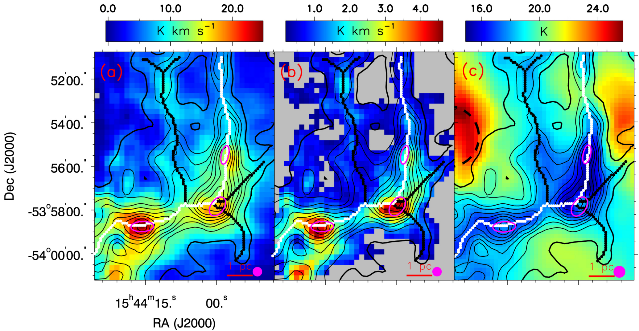
Figure 3. from Yu-Xin He et al 2023 Astrophys. J. 957 doi:10.3847/1538-4357/acf766 https://dx.doi.org/10.3847/1538-4357/acf766 © 2023. The Author(s). Published by the American Astronomical Society.
