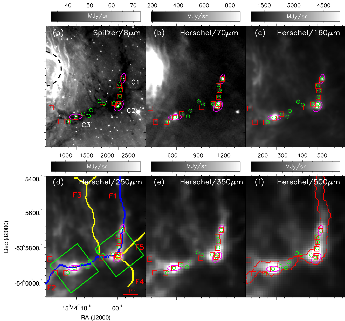
Figure 1. from Yu-Xin He et al 2023 Astrophys. J. 957 doi:10.3847/1538-4357/acf766 https://dx.doi.org/10.3847/1538-4357/acf766 © 2023. The Author(s). Published by the American Astronomical Society.
