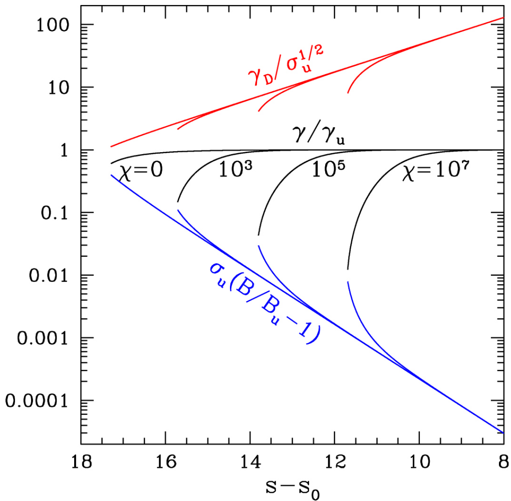
Figure 8. from Andrei M. Beloborodov 2023 Astrophys. J. 959 doi:10.3847/1538-4357/acf659 https://dx.doi.org/10.3847/1538-4357/acf659 © 2023. The Author(s). Published by the American Astronomical Society.
