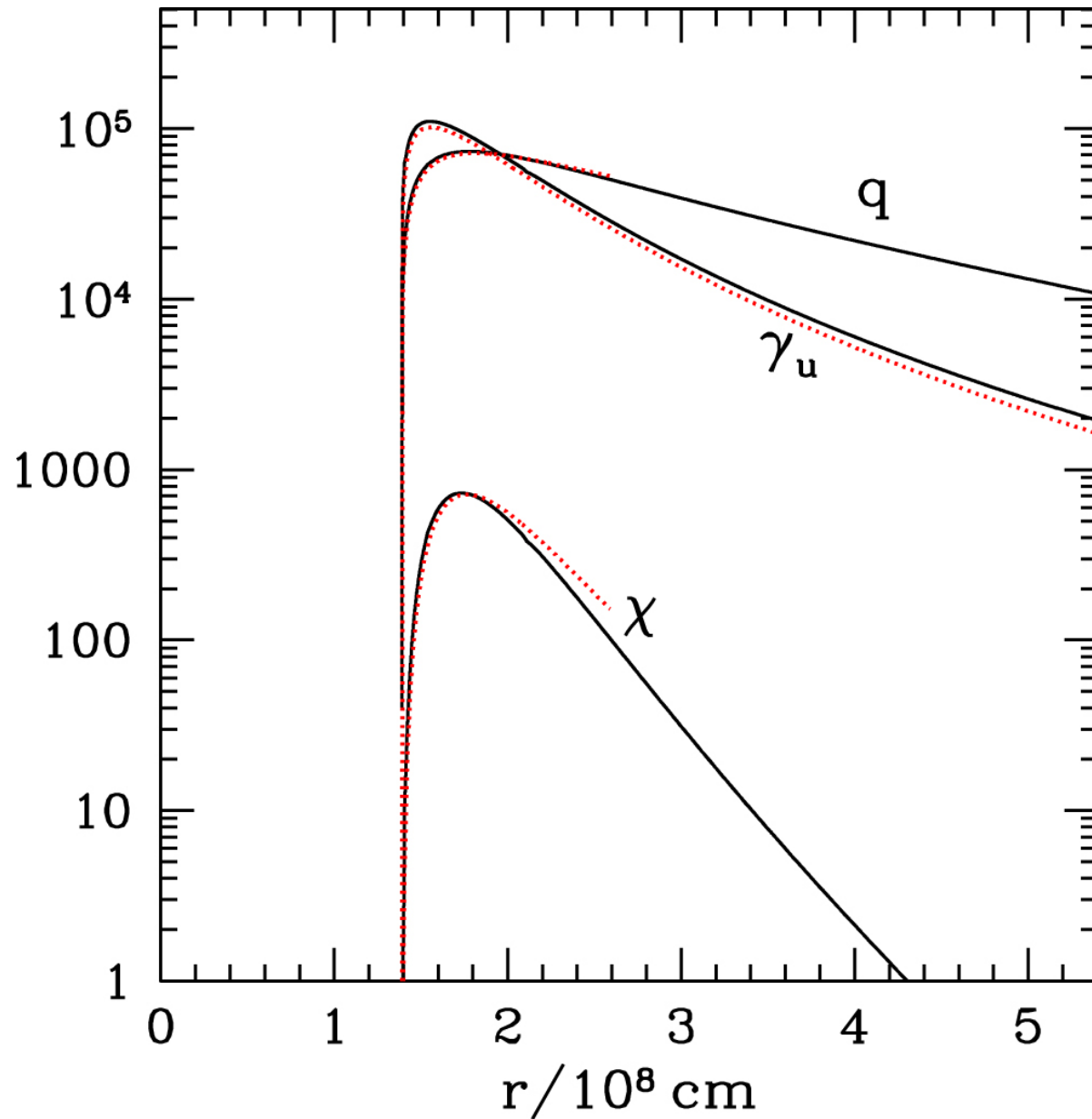
Figure 6. from Andrei M. Beloborodov 2023 Astrophys. J. 959 doi:10.3847/1538-4357/acf659 https://dx.doi.org/10.3847/1538-4357/acf659 © 2023. The Author(s). Published by the American Astronomical Society.
