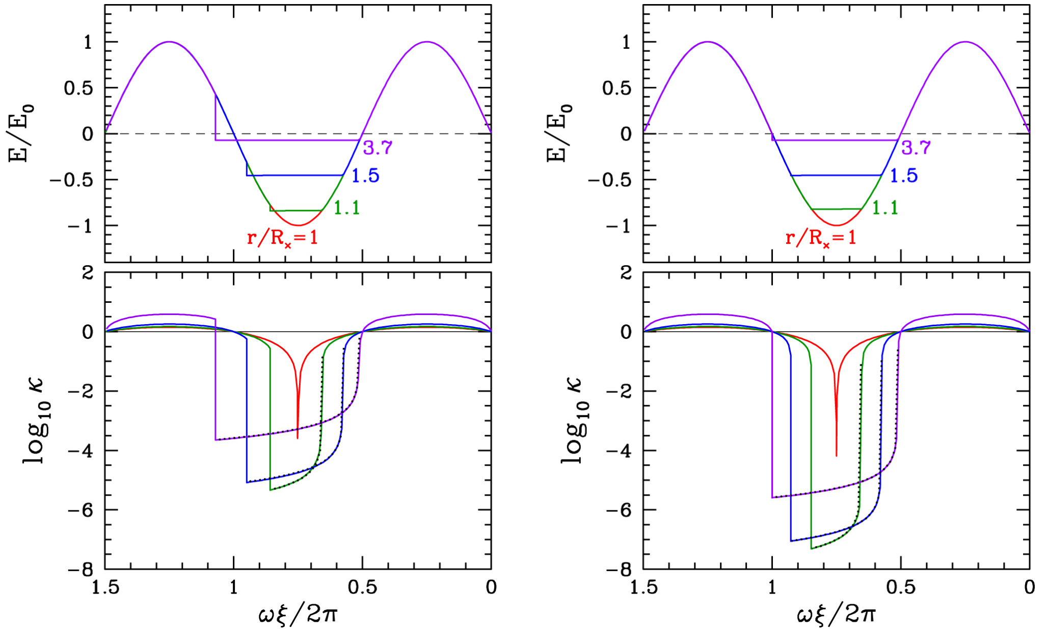
Figure 5. from Andrei M. Beloborodov 2023 Astrophys. J. 959 doi:10.3847/1538-4357/acf659 https://dx.doi.org/10.3847/1538-4357/acf659 © 2023. The Author(s). Published by the American Astronomical Society.
