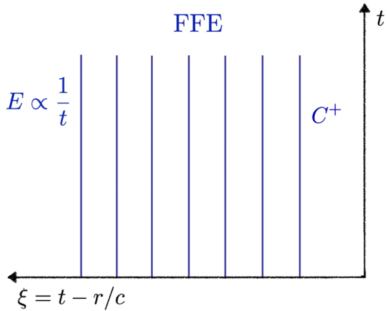
Figure 3. from Andrei M. Beloborodov 2023 Astrophys. J. 959 doi:10.3847/1538-4357/acf659 https://dx.doi.org/10.3847/1538-4357/acf659 © 2023. The Author(s). Published by the American Astronomical Society.
