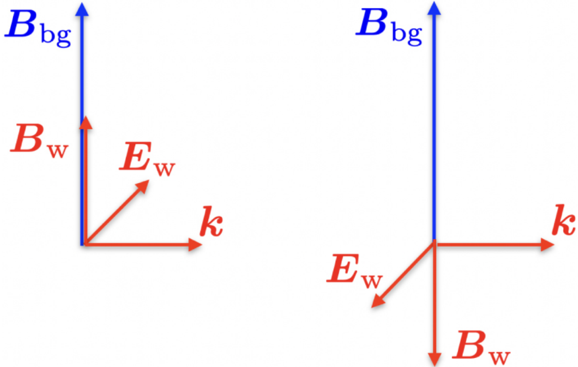
Figure 2. from Andrei M. Beloborodov 2023 Astrophys. J. 959 doi:10.3847/1538-4357/acf659 https://dx.doi.org/10.3847/1538-4357/acf659 © 2023. The Author(s). Published by the American Astronomical Society.
