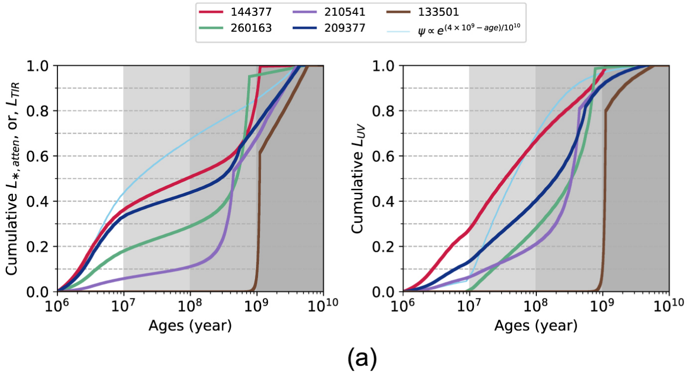
Figure 10. from Po-Feng Wu et al 2023 Astrophys. J. 955 doi:10.3847/1538-4357/acf0bd https://dx.doi.org/10.3847/1538-4357/acf0bd © 2023. The Author(s). Published by the American Astronomical Society.
