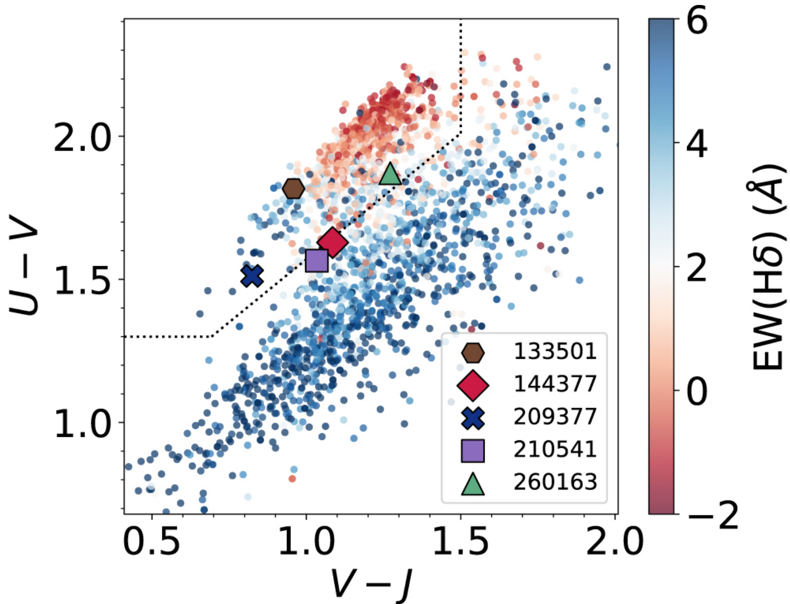
Figure 1. from Po-Feng Wu et al 2023 Astrophys. J. 955 doi:10.3847/1538-4357/acf0bd https://dx.doi.org/10.3847/1538-4357/acf0bd © 2023. The Author(s). Published by the American Astronomical Society.
