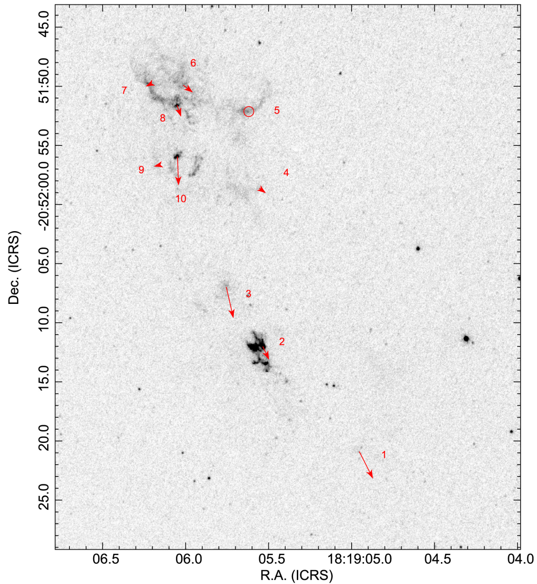
Figure 9. from John Bally and Bo Reipurth 2023 Astrophys. J. 958 doi:10.3847/1538-4357/acf028 https://dx.doi.org/10.3847/1538-4357/acf028 © 2023. The Author(s). Published by the American Astronomical Society.
