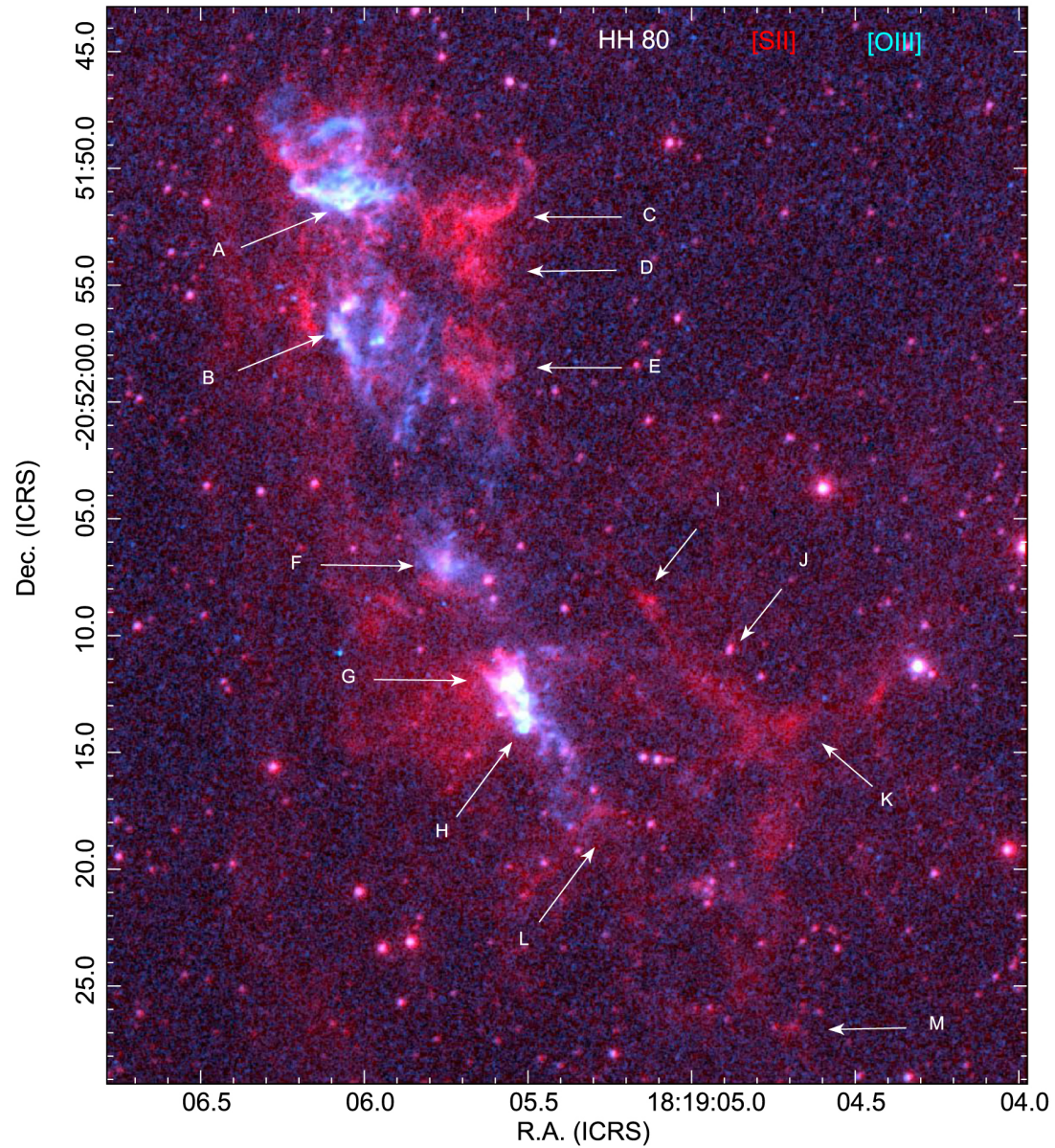
Figure 6. from John Bally and Bo Reipurth 2023 Astrophys. J. 958 doi:10.3847/1538-4357/acf028 https://dx.doi.org/10.3847/1538-4357/acf028 © 2023. The Author(s). Published by the American Astronomical Society.
