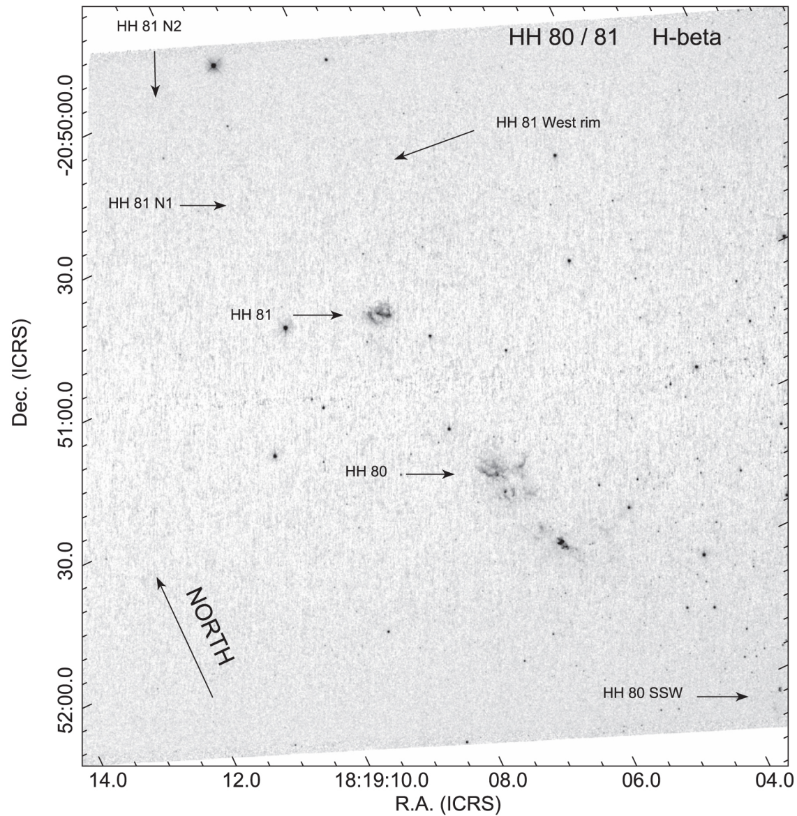
Figure 4. from John Bally and Bo Reipurth 2023 Astrophys. J. 958 doi:10.3847/1538-4357/acf028 https://dx.doi.org/10.3847/1538-4357/acf028 © 2023. The Author(s). Published by the American Astronomical Society.
