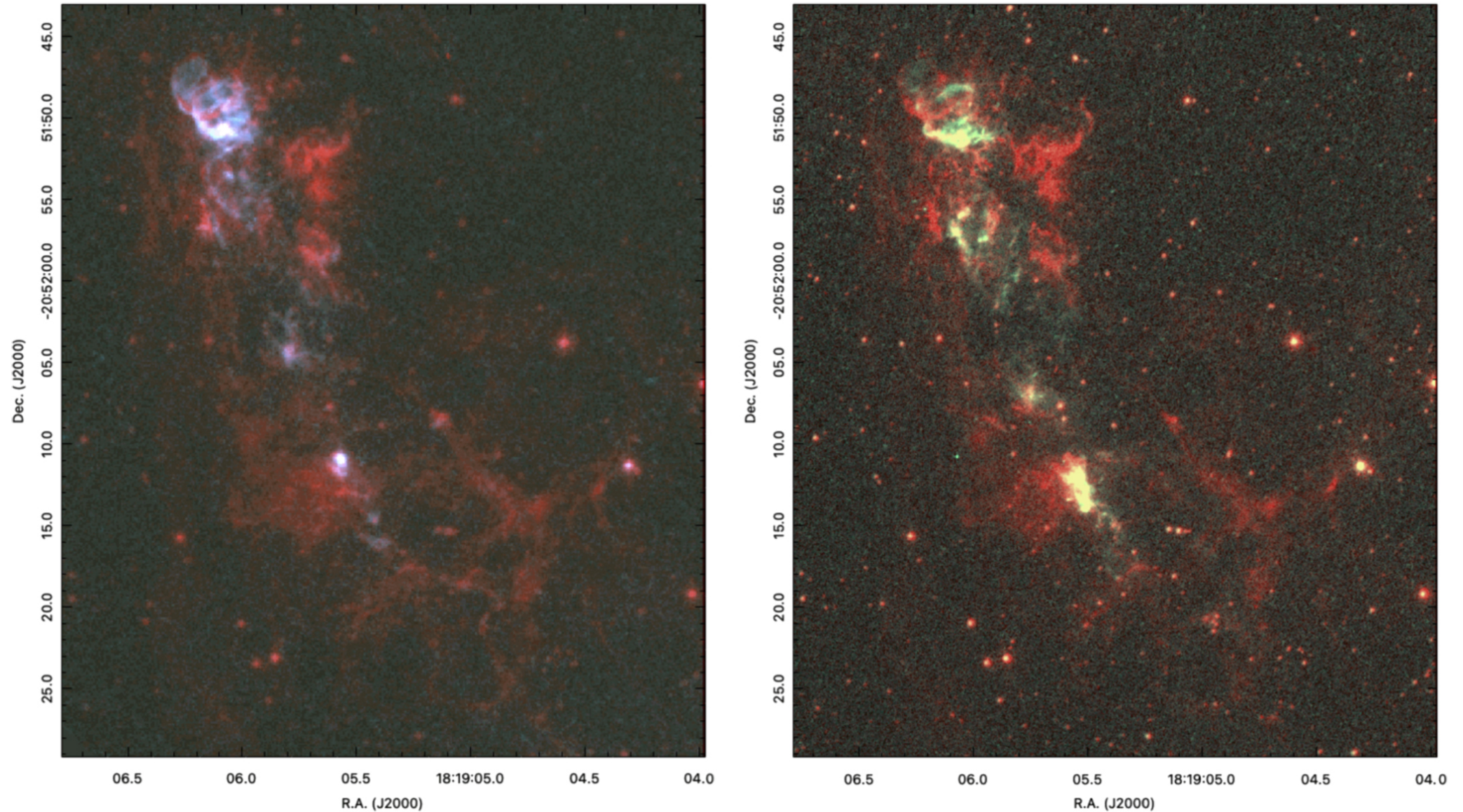
Figure 25. from John Bally and Bo Reipurth 2023 Astrophys. J. 958 doi:10.3847/1538-4357/acf028 https://dx.doi.org/10.3847/1538-4357/acf028 © 2023. The Author(s). Published by the American Astronomical Society.
