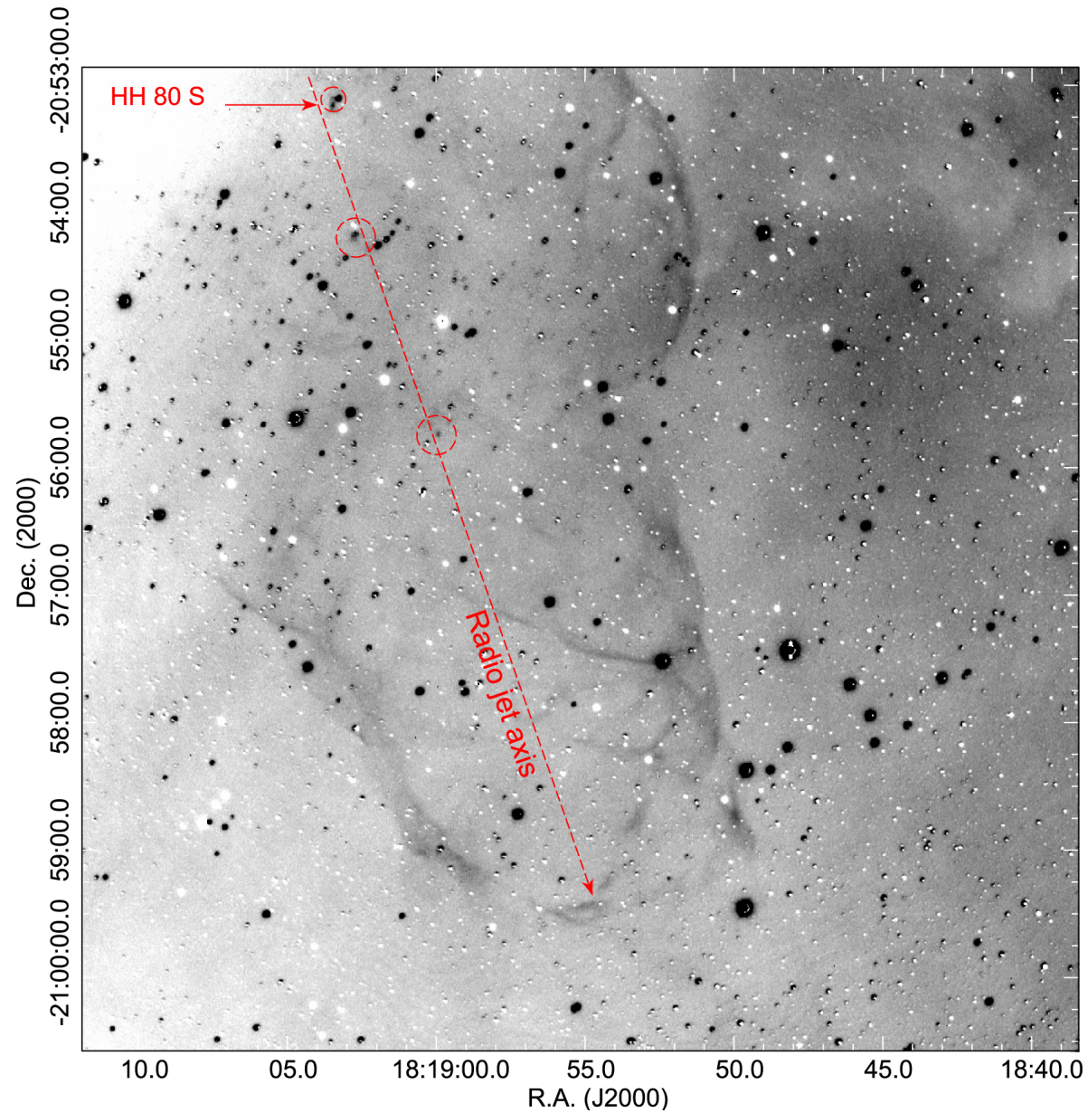
Figure 13. from John Bally and Bo Reipurth 2023 Astrophys. J. 958 doi:10.3847/1538-4357/acf028 https://dx.doi.org/10.3847/1538-4357/acf028 © 2023. The Author(s). Published by the American Astronomical Society.
