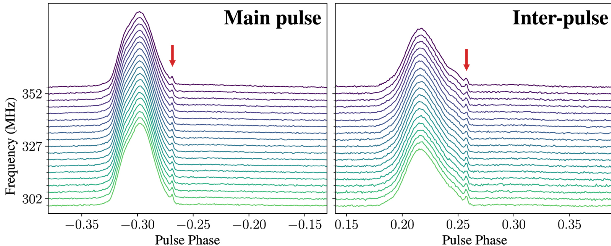
Figure 8. from Nikhil Mahajan and Marten H. van Kerkwijk 2023 Astrophys. J. 955 doi:10.3847/1538-4357/acec3a https://dx.doi.org/10.3847/1538-4357/acec3a © 2023. The Author(s). Published by the American Astronomical Society.
