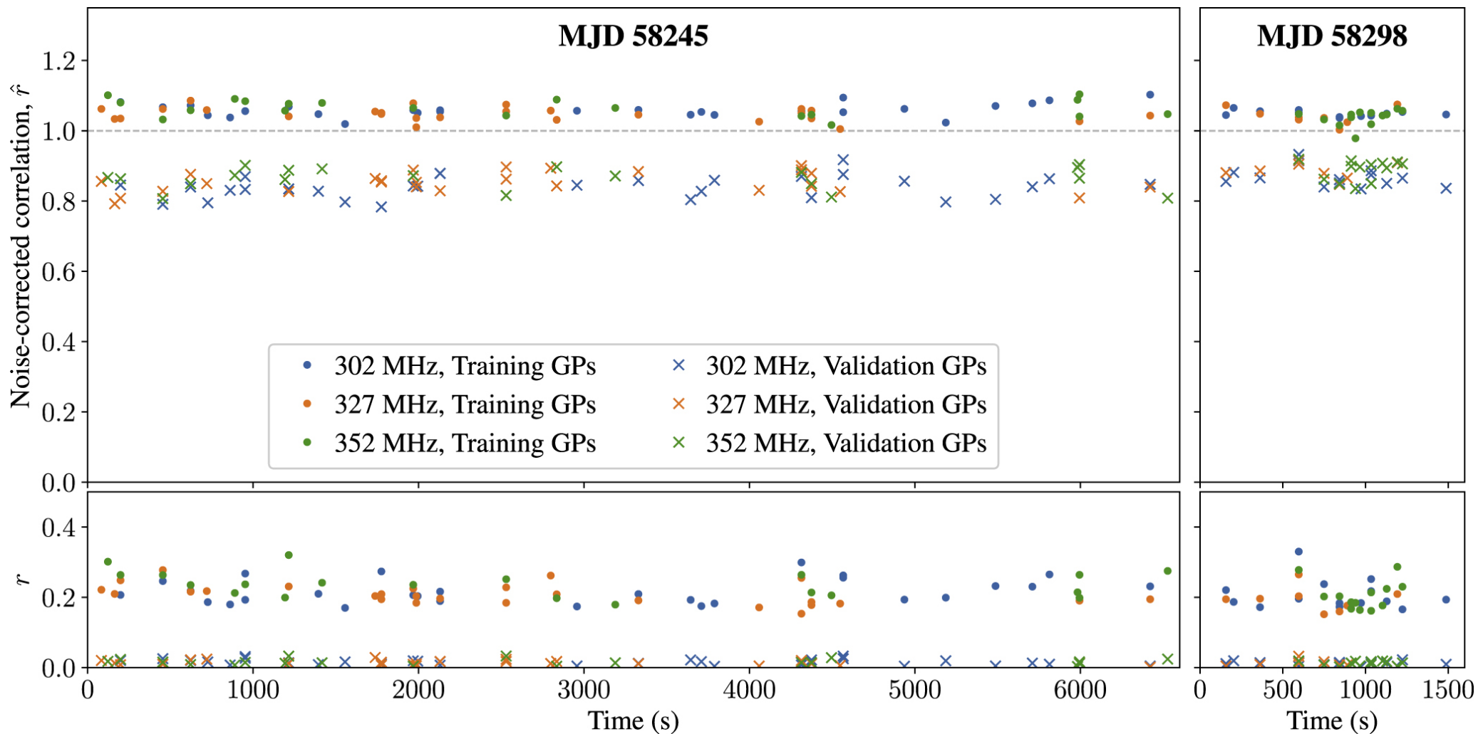
Figure 6. from Nikhil Mahajan and Marten H. van Kerkwijk 2023 Astrophys. J. 955 doi:10.3847/1538-4357/acec3a https://dx.doi.org/10.3847/1538-4357/acec3a © 2023. The Author(s). Published by the American Astronomical Society.
