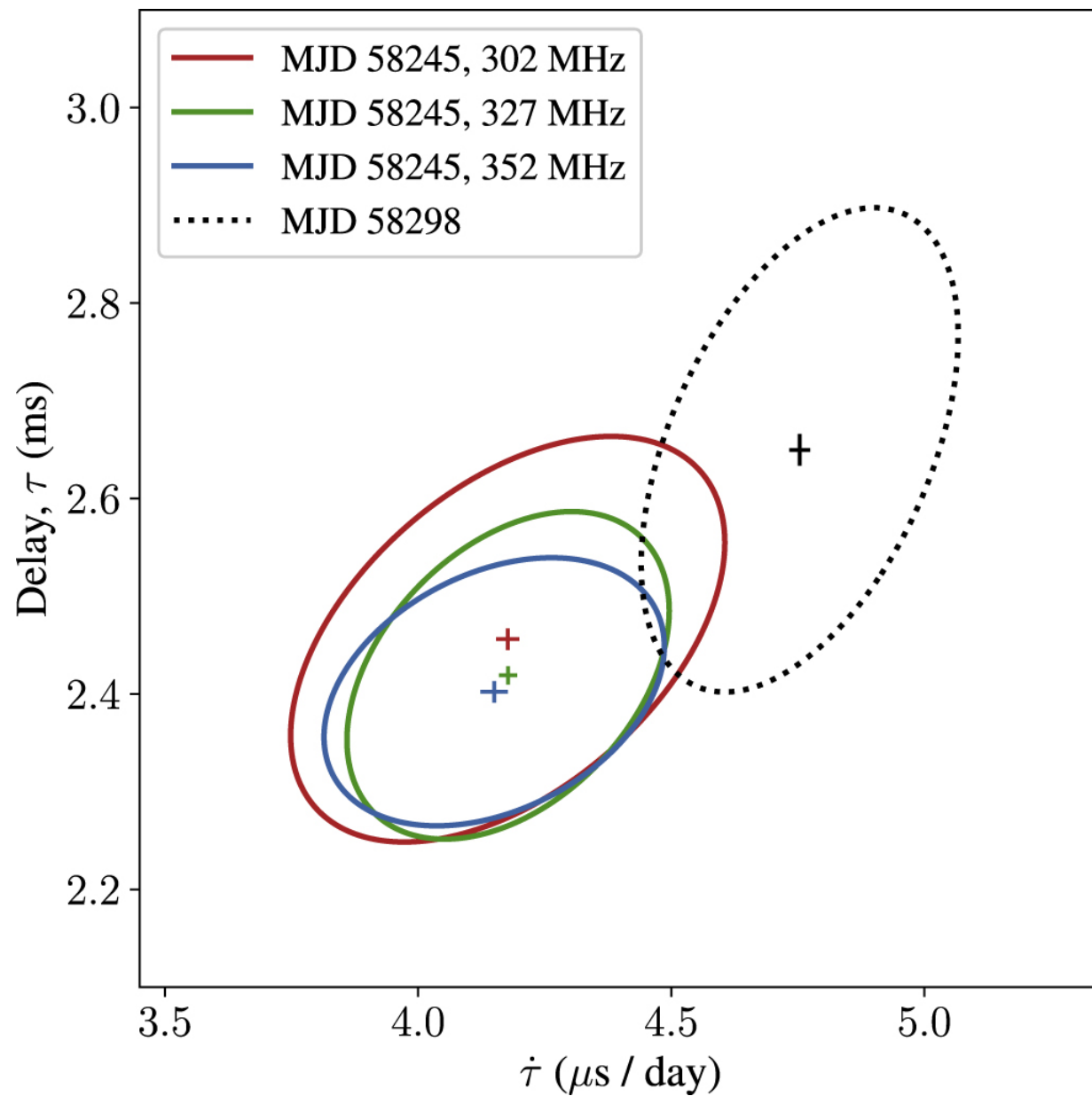
Figure 5. from Nikhil Mahajan and Marten H. van Kerkwijk 2023 Astrophys. J. 955 doi:10.3847/1538-4357/acec3a https://dx.doi.org/10.3847/1538-4357/acec3a © 2023. The Author(s). Published by the American Astronomical Society.
