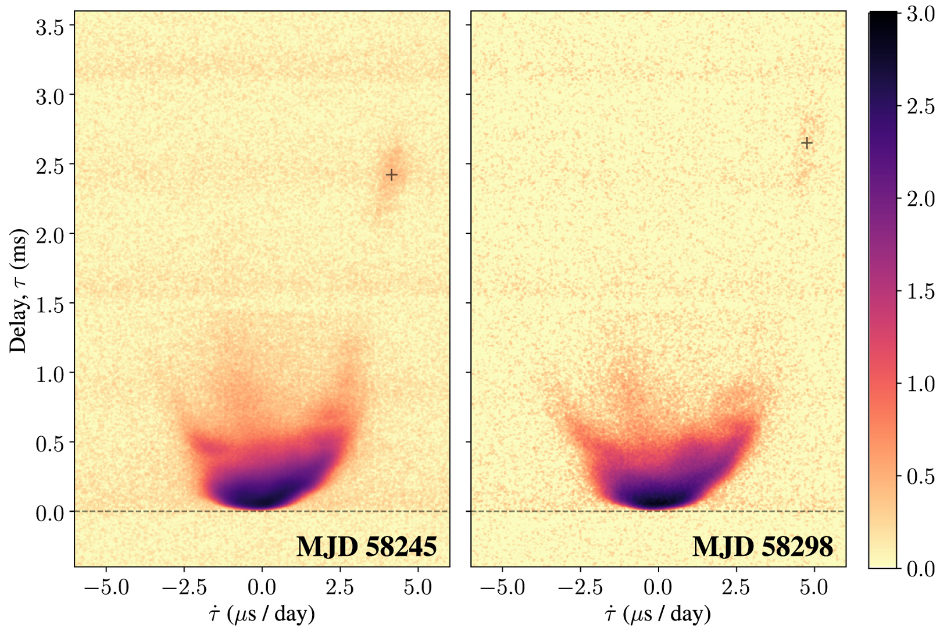
Figure 4. from Nikhil Mahajan and Marten H. van Kerkwijk 2023 Astrophys. J. 955 doi:10.3847/1538-4357/acec3a https://dx.doi.org/10.3847/1538-4357/acec3a © 2023. The Author(s). Published by the American Astronomical Society.
