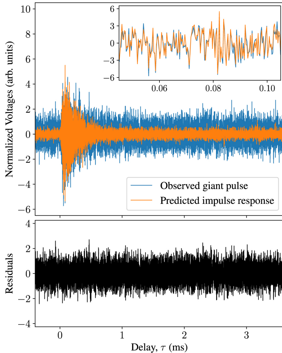
Figure 3. from Nikhil Mahajan and Marten H. van Kerkwijk 2023 Astrophys. J. 955 doi:10.3847/1538-4357/acec3a https://dx.doi.org/10.3847/1538-4357/acec3a © 2023. The Author(s). Published by the American Astronomical Society.
