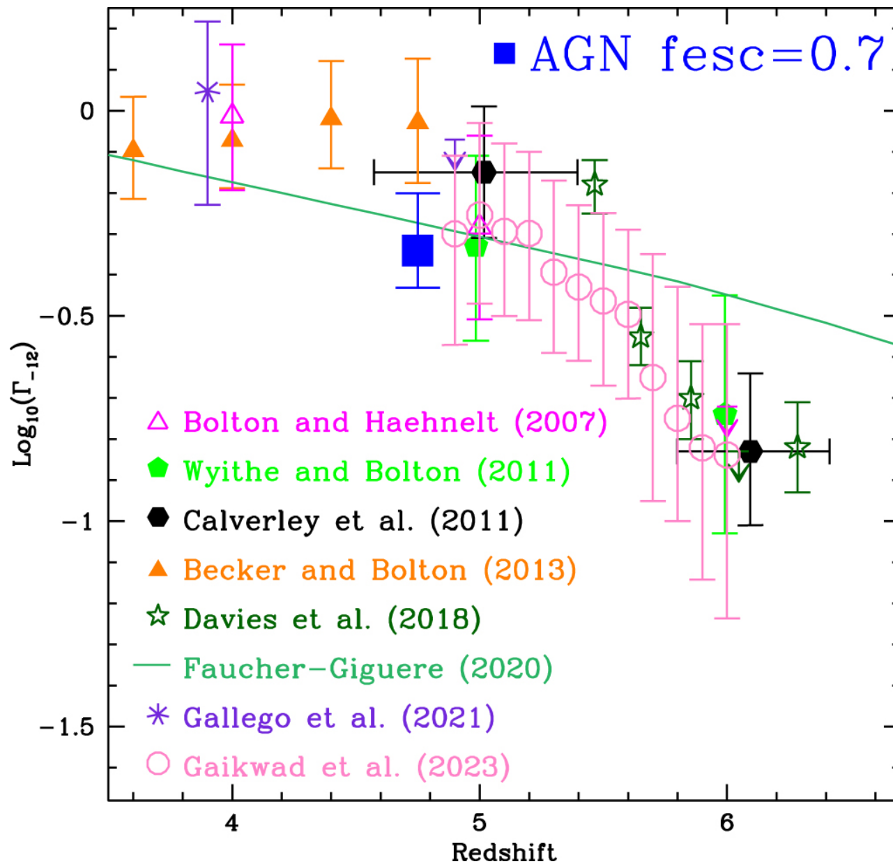
Figure 7. from Andrea Grazian et al 2023 Astrophys. J. 955 doi:10.3847/1538-4357/aceb60 https://dx.doi.org/10.3847/1538-4357/aceb60 © 2023. The Author(s). Published by the American Astronomical Society.
