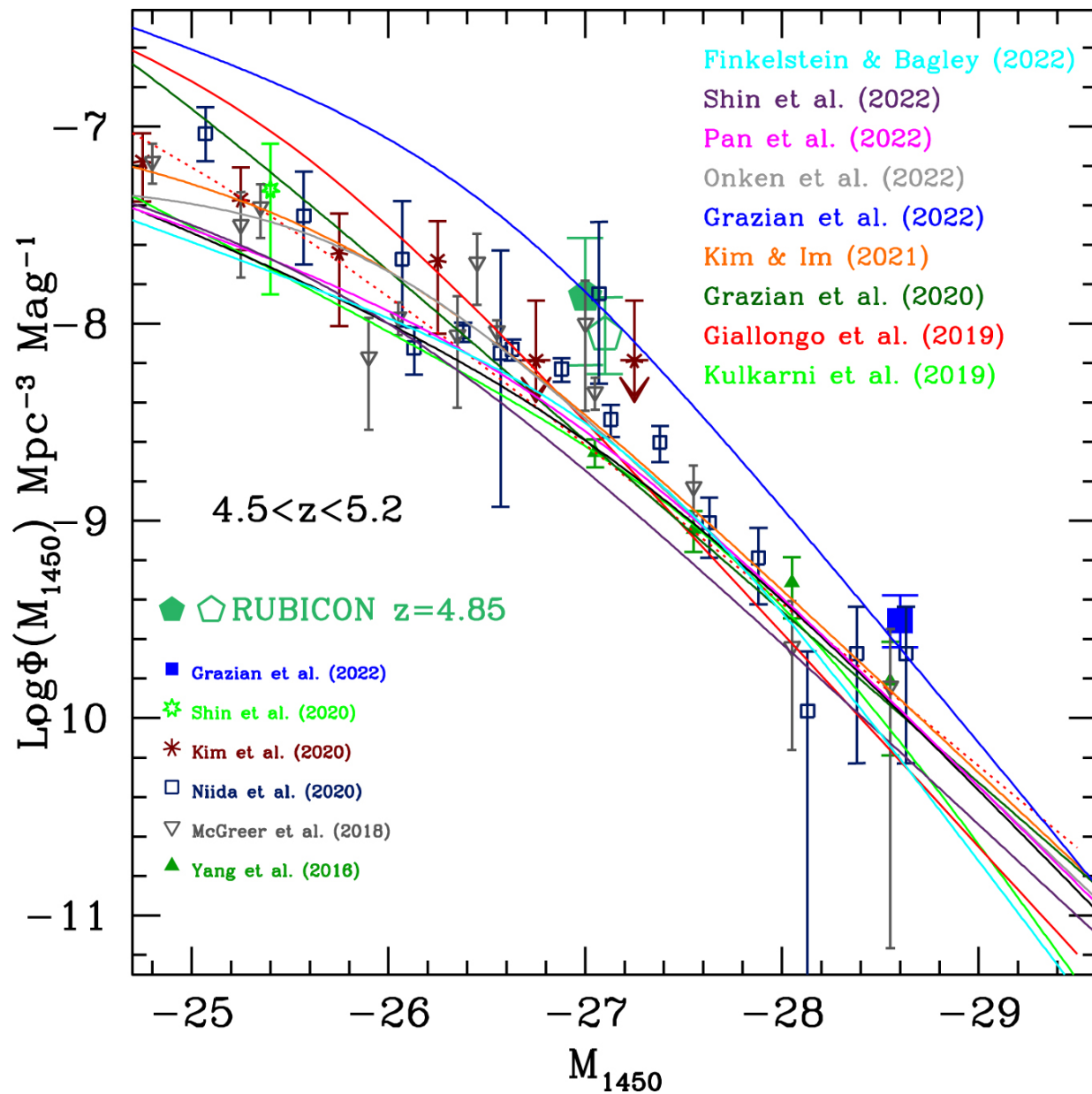
Figure 6. from Andrea Grazian et al 2023 Astrophys. J. 955 doi:10.3847/1538-4357/aceb60 https://dx.doi.org/10.3847/1538-4357/aceb60 © 2023. The Author(s). Published by the American Astronomical Society.
