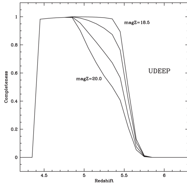
Figure 5. from Andrea Grazian et al 2023 Astrophys. J. 955 doi:10.3847/1538-4357/aceb60 https://dx.doi.org/10.3847/1538-4357/aceb60 © 2023. The Author(s). Published by the American Astronomical Society.
