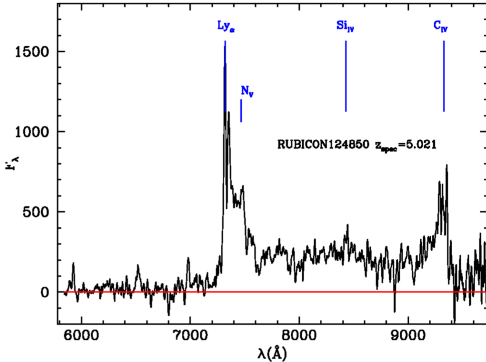
Figure 4. from Andrea Grazian et al 2023 Astrophys. J. 955 doi:10.3847/1538-4357/aceb60 https://dx.doi.org/10.3847/1538-4357/aceb60 © 2023. The Author(s). Published by the American Astronomical Society.
