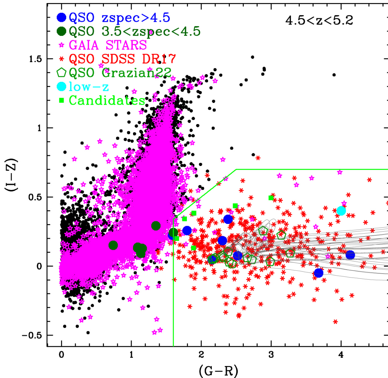
Figure 3. from Andrea Grazian et al 2023 Astrophys. J. 955 doi:10.3847/1538-4357/aceb60 https://dx.doi.org/10.3847/1538-4357/aceb60 © 2023. The Author(s). Published by the American Astronomical Society.
