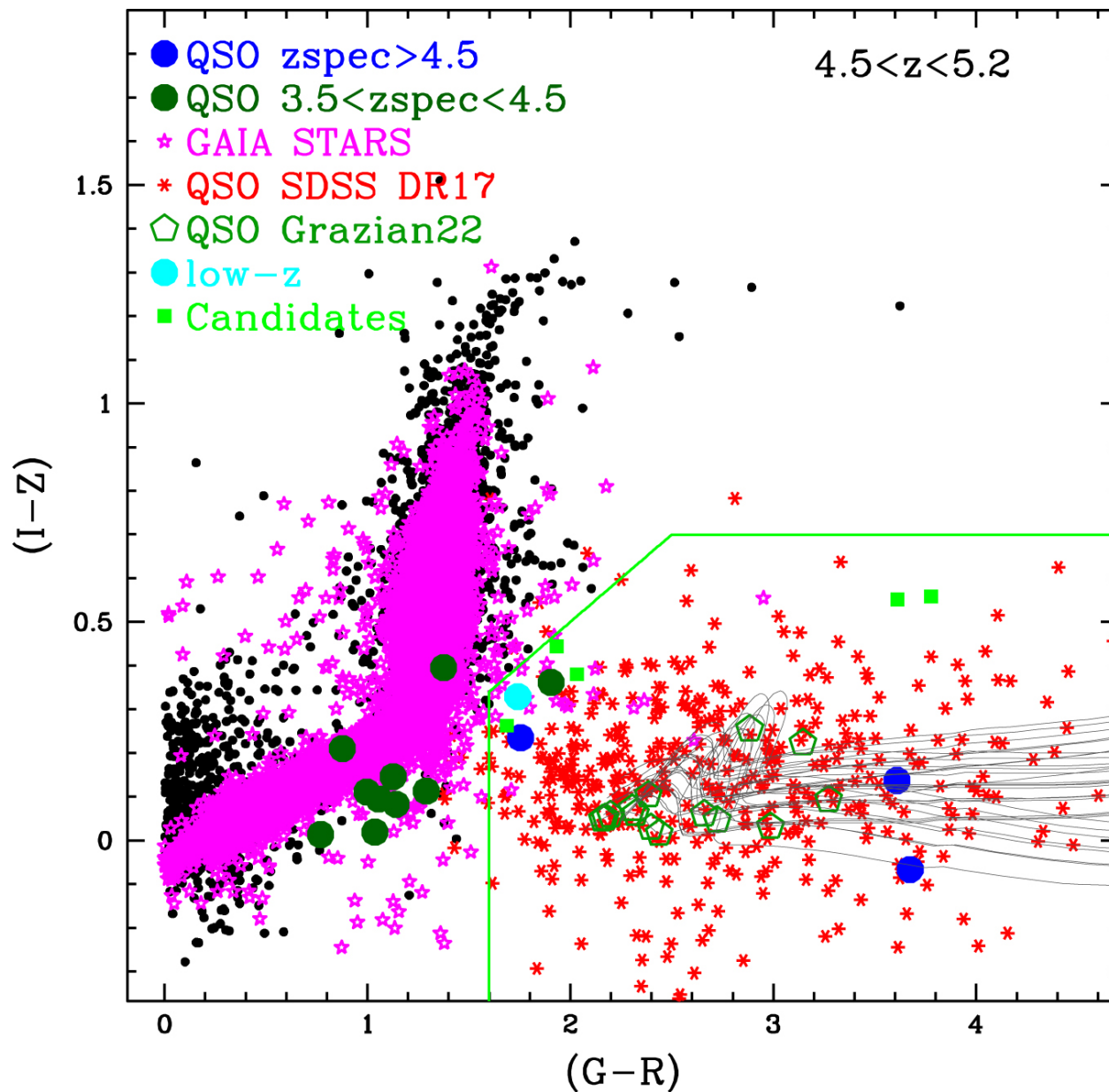
Figure 1. from Andrea Grazian et al 2023 Astrophys. J. 955 doi:10.3847/1538-4357/aceb60 https://dx.doi.org/10.3847/1538-4357/aceb60 © 2023. The Author(s). Published by the American Astronomical Society.
