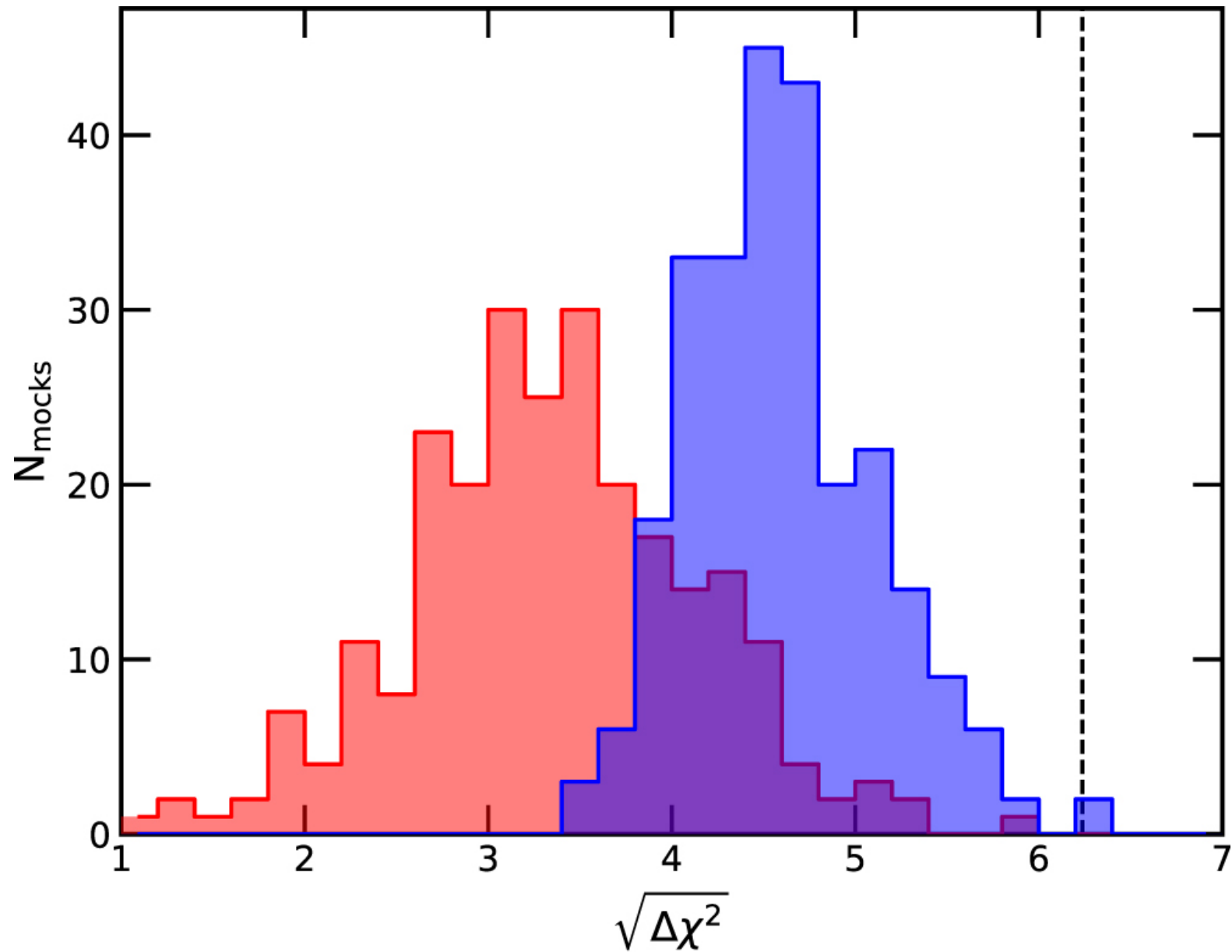
Figure 8. from R. Brent Tully et al 2023 Astrophys. J. 954 doi:10.3847/1538-4357/aceaf3 https://dx.doi.org/10.3847/1538-4357/aceaf3 © 2023. The Author(s). Published by the American Astronomical Society.
