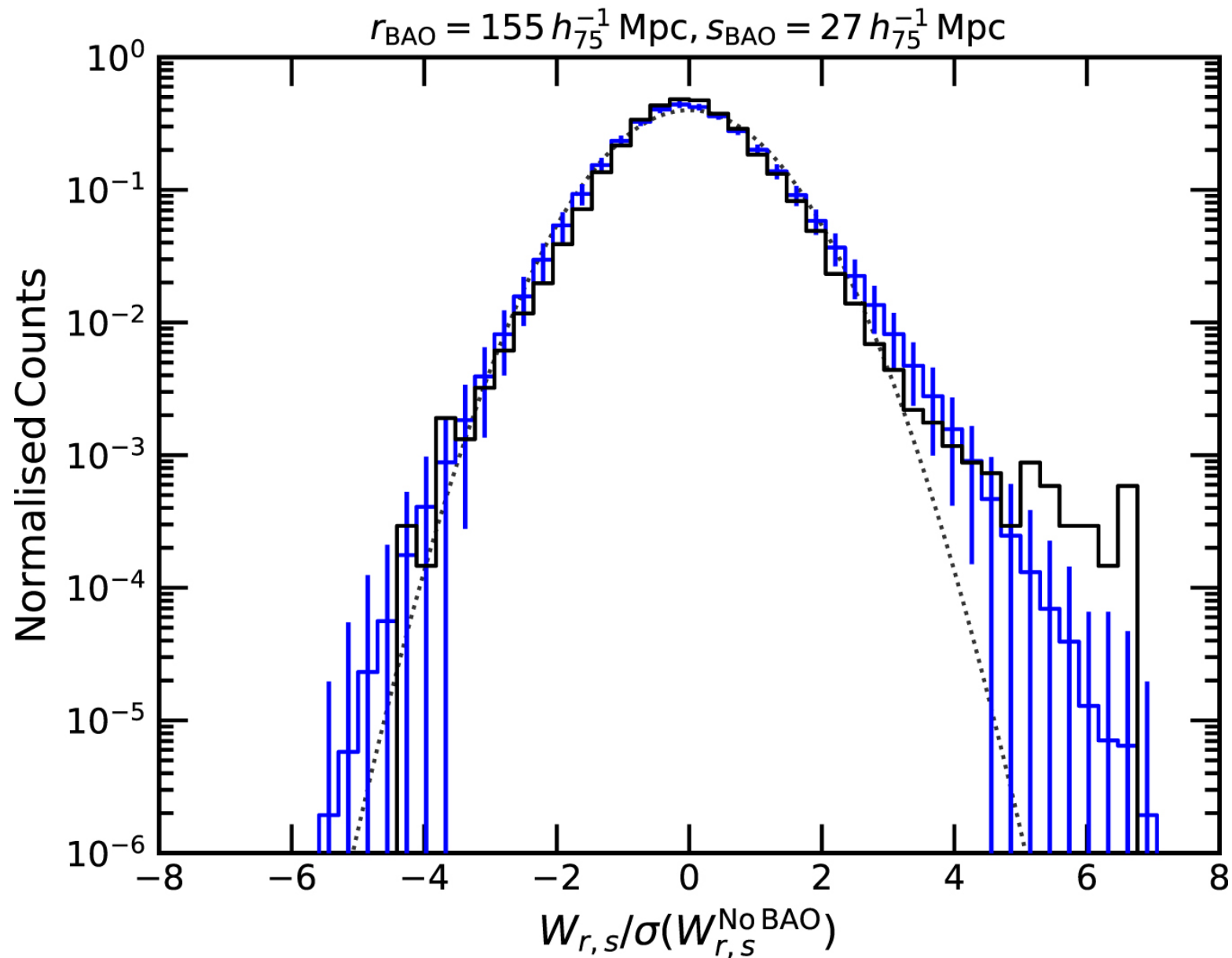
Figure 7. from R. Brent Tully et al 2023 Astrophys. J. 954 doi:10.3847/1538-4357/aceaf3 https://dx.doi.org/10.3847/1538-4357/aceaf3 © 2023. The Author(s). Published by the American Astronomical Society.
