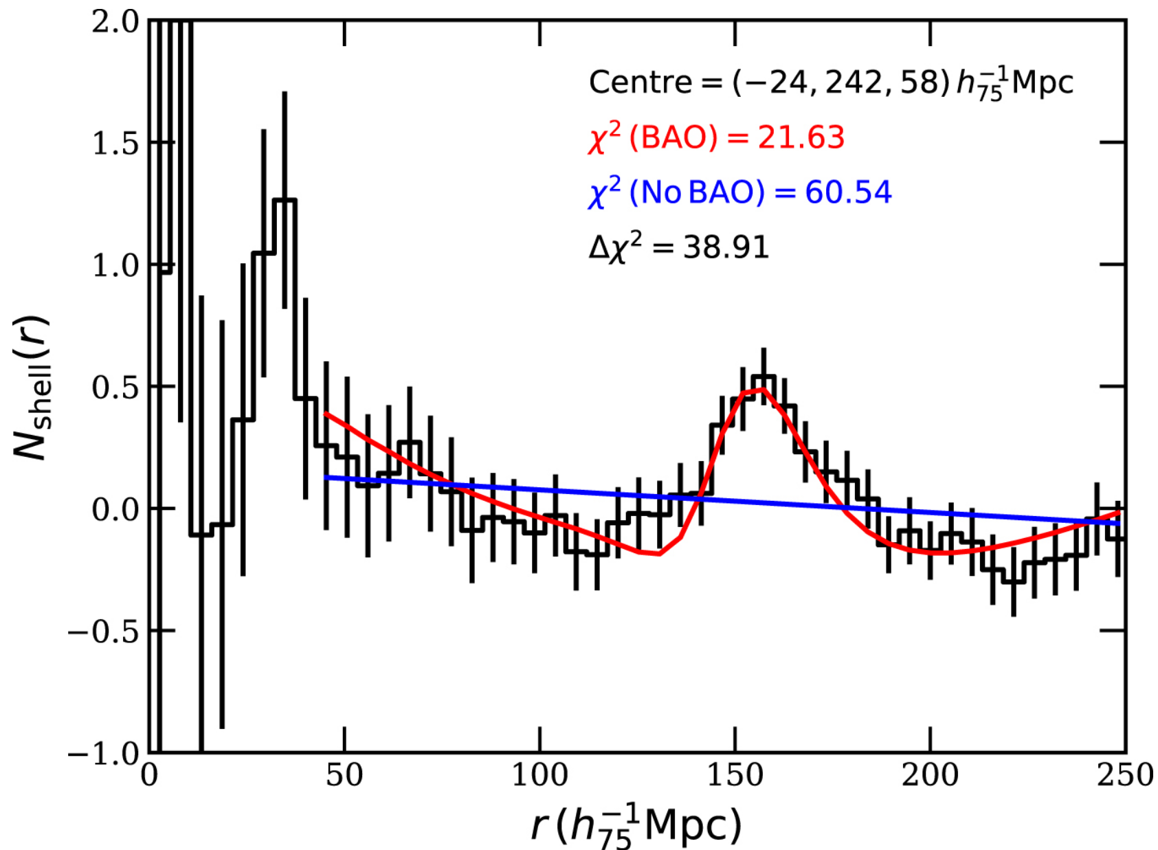
Figure 5. from R. Brent Tully et al 2023 Astrophys. J. 954 doi:10.3847/1538-4357/aceaf3 https://dx.doi.org/10.3847/1538-4357/aceaf3 © 2023. The Author(s). Published by the American Astronomical Society.
