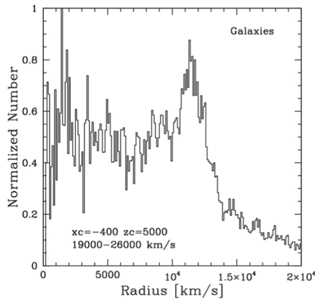
Figure 3. from R. Brent Tully et al 2023 Astrophys. J. 954 doi:10.3847/1538-4357/aceaf3 https://dx.doi.org/10.3847/1538-4357/aceaf3 © 2023. The Author(s). Published by the American Astronomical Society.
