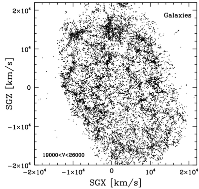
Figure 2. from R. Brent Tully et al 2023 Astrophys. J. 954 doi:10.3847/1538-4357/aceaf3 https://dx.doi.org/10.3847/1538-4357/aceaf3 © 2023. The Author(s). Published by the American Astronomical Society.
