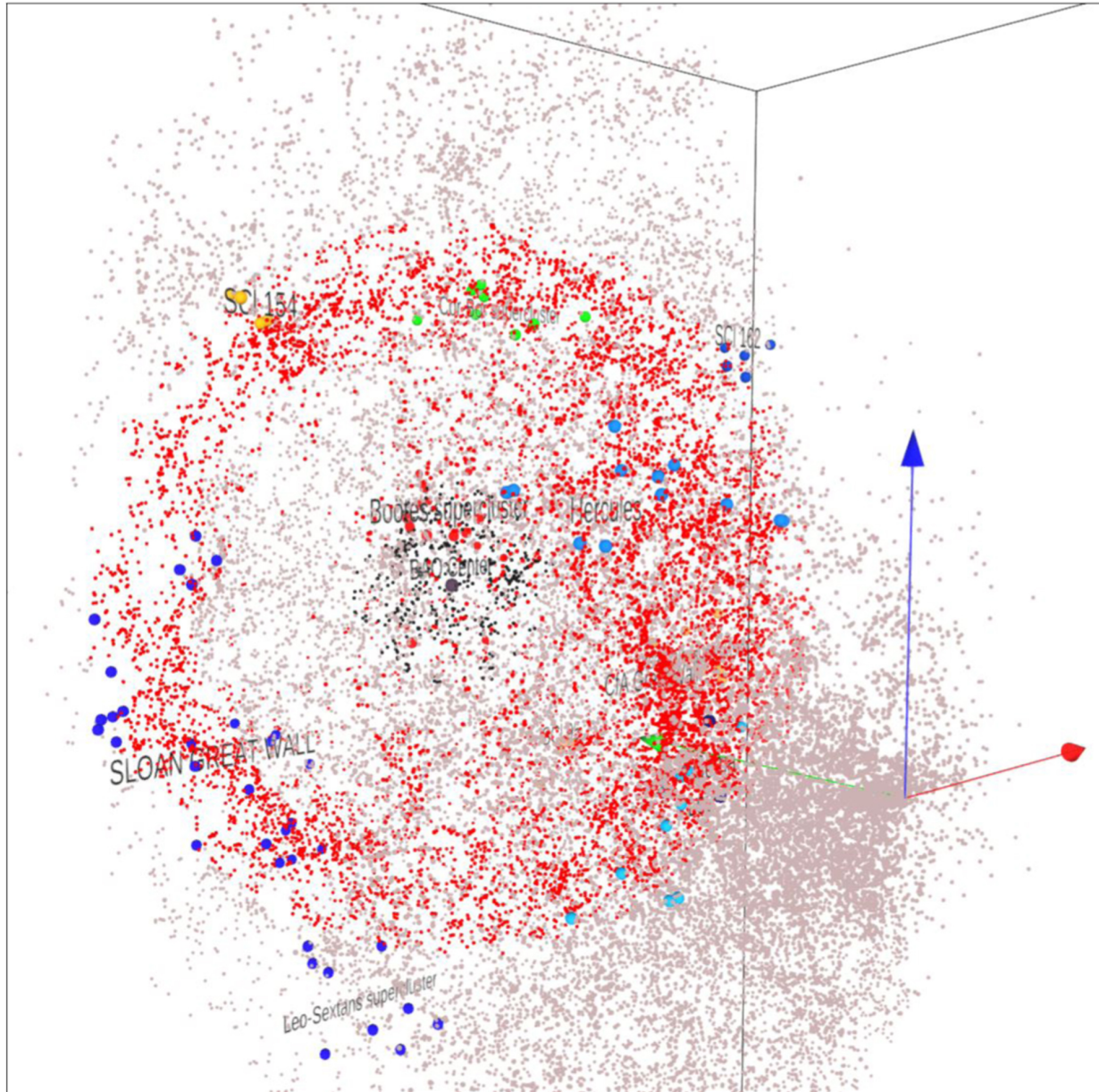
Figure 13. from R. Brent Tully et al 2023 Astrophys. J. 954 doi:10.3847/1538-4357/aceaf3 https://dx.doi.org/10.3847/1538-4357/aceaf3 © 2023. The Author(s). Published by the American Astronomical Society.
