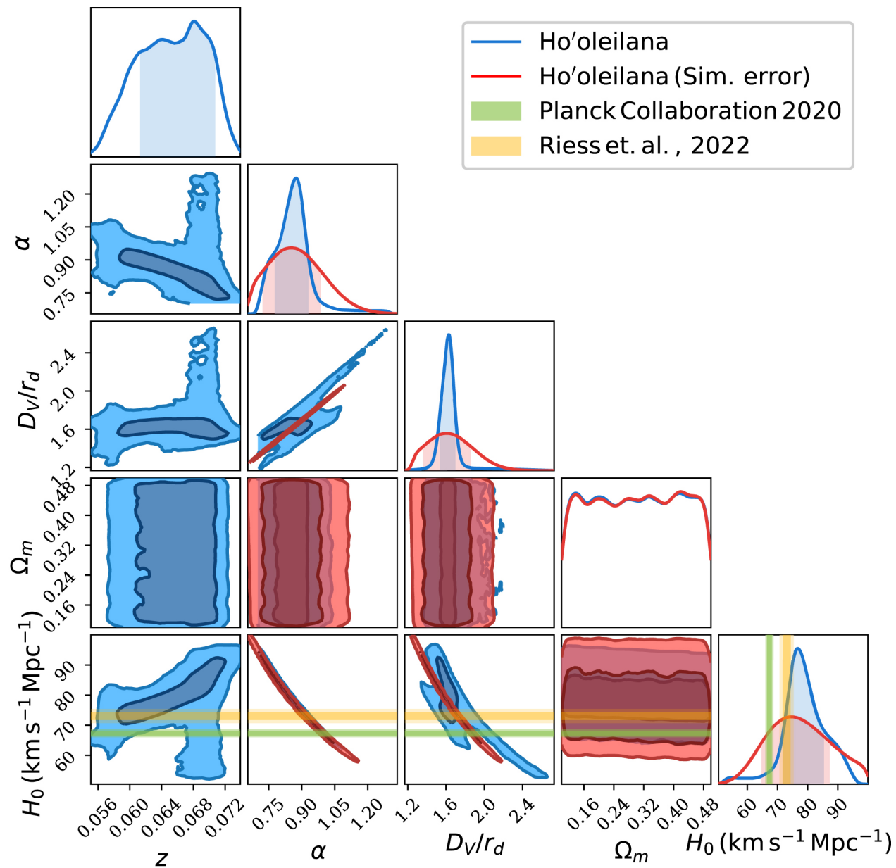
Figure 10. from R. Brent Tully et al 2023 Astrophys. J. 954 doi:10.3847/1538-4357/aceaf3 https://dx.doi.org/10.3847/1538-4357/aceaf3 © 2023. The Author(s). Published by the American Astronomical Society.
