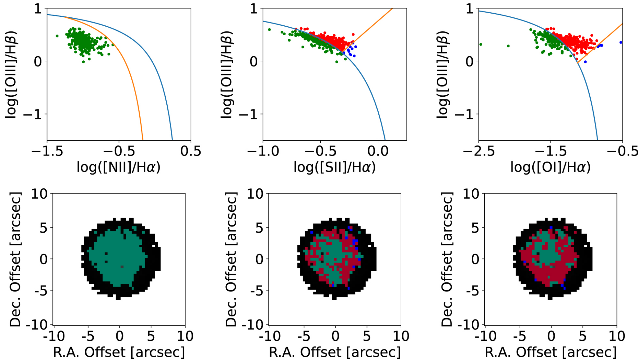
Figure 9. from Victor D. Johnston et al 2023 Astrophys. J. 954 doi:10.3847/1538-4357/ace90e https://dx.doi.org/10.3847/1538-4357/ace90e © 2023. The Author(s). Published by the American Astronomical Society.
