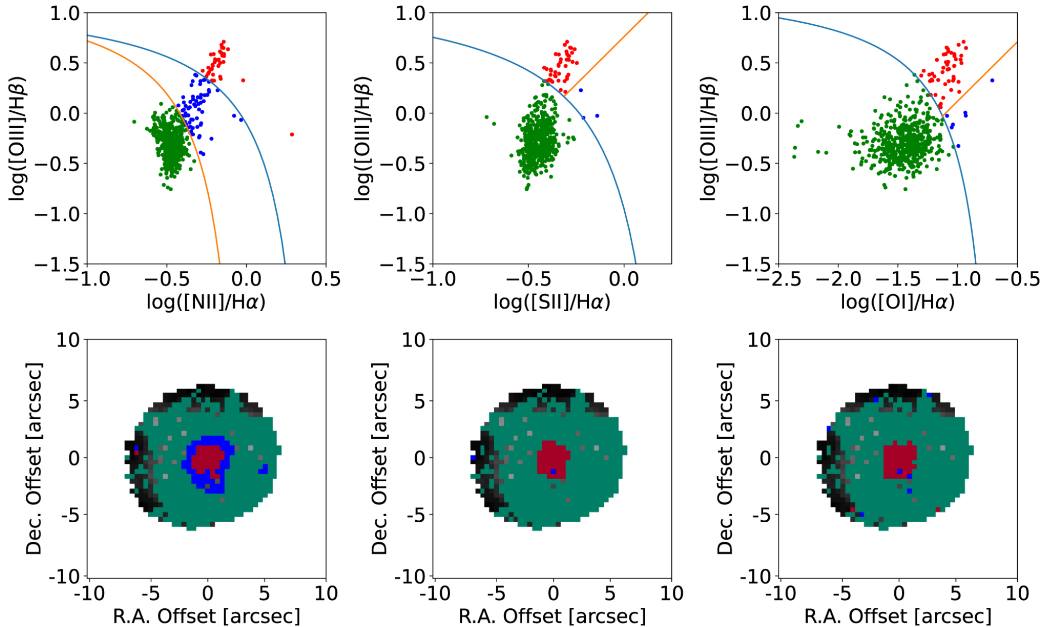
Figure 4. from Victor D. Johnston et al 2023 Astrophys. J. 954 doi:10.3847/1538-4357/ace90e https://dx.doi.org/10.3847/1538-4357/ace90e © 2023. The Author(s). Published by the American Astronomical Society.
