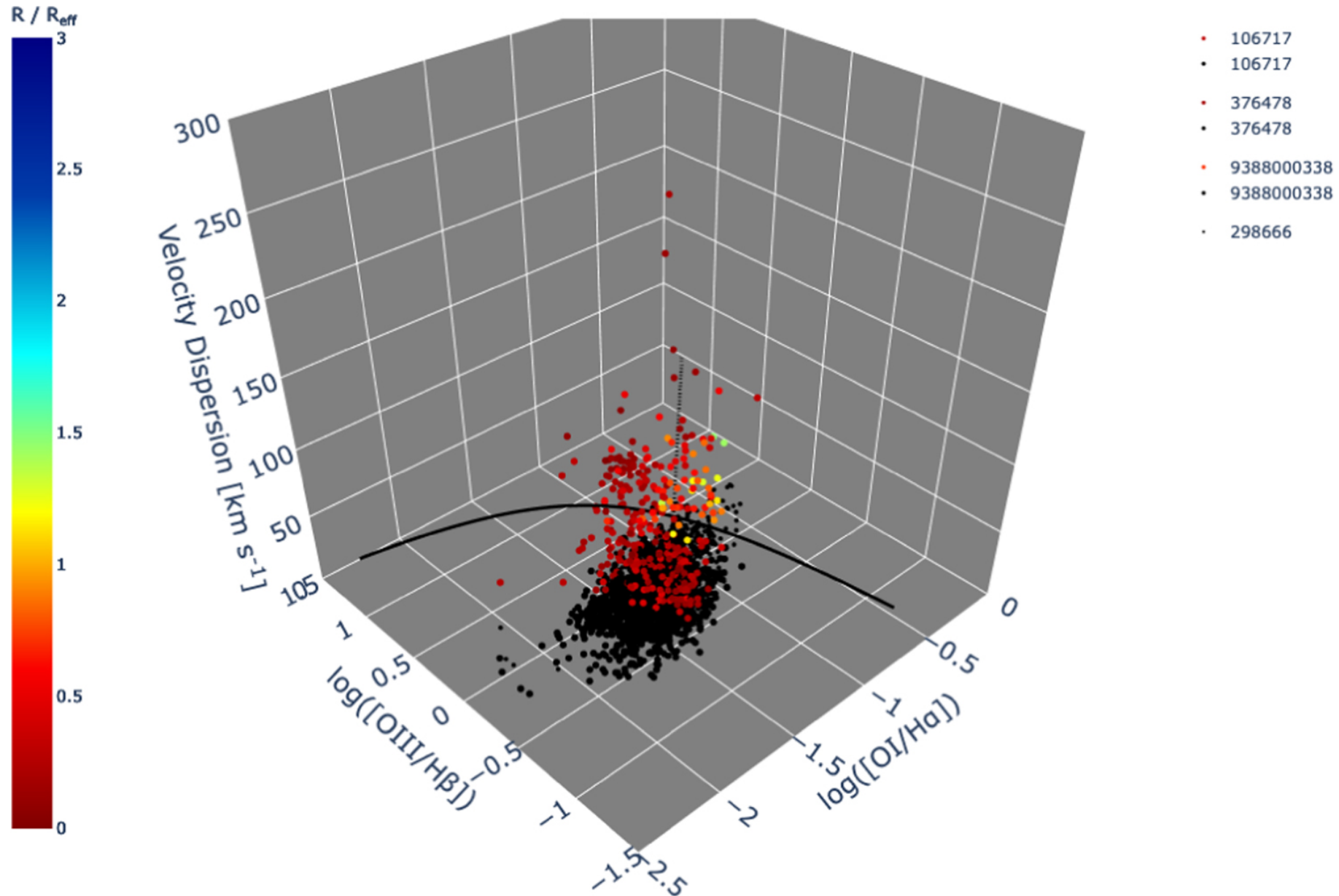
Figure 15. from Victor D. Johnston et al 2023 Astrophys. J. 954 doi:10.3847/1538-4357/ace90e https://dx.doi.org/10.3847/1538-4357/ace90e © 2023. The Author(s). Published by the American Astronomical Society.
