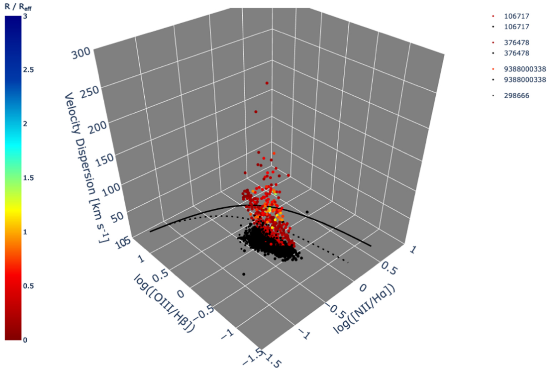
Figure 13. from Victor D. Johnston et al 2023 Astrophys. J. 954 doi:10.3847/1538-4357/ace90e https://dx.doi.org/10.3847/1538-4357/ace90e © 2023. The Author(s). Published by the American Astronomical Society.
