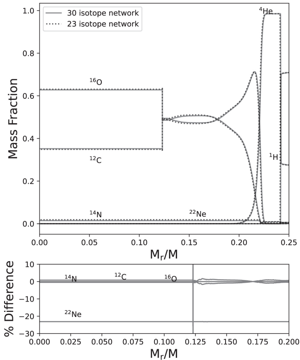
Figure 9. from Morgan T. Chidester et al 2023 Astrophys. J. 954 doi:10.3847/1538-4357/ace620 https://dx.doi.org/10.3847/1538-4357/ace620 © 2023. The Author(s). Published by the American Astronomical Society.
