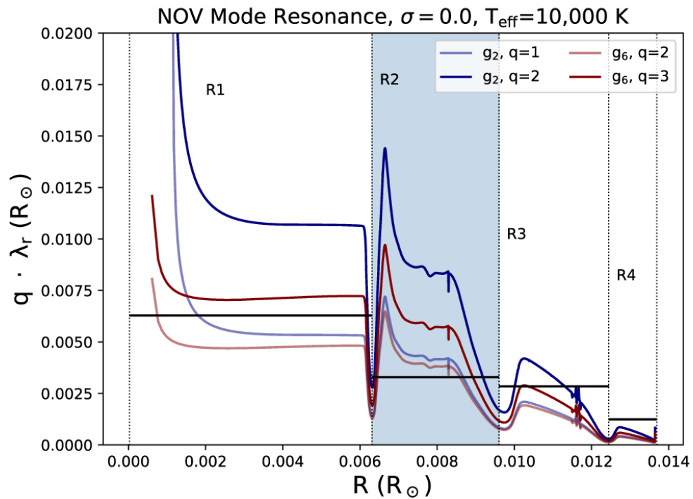
Figure 7. from Morgan T. Chidester et al 2023 Astrophys. J. 954 doi:10.3847/1538-4357/ace620 https://dx.doi.org/10.3847/1538-4357/ace620 © 2023. The Author(s). Published by the American Astronomical Society.
