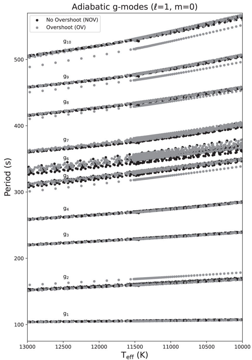
Figure 5. from Morgan T. Chidester et al 2023 Astrophys. J. 954 doi:10.3847/1538-4357/ace620 https://dx.doi.org/10.3847/1538-4357/ace620 © 2023. The Author(s). Published by the American Astronomical Society.
