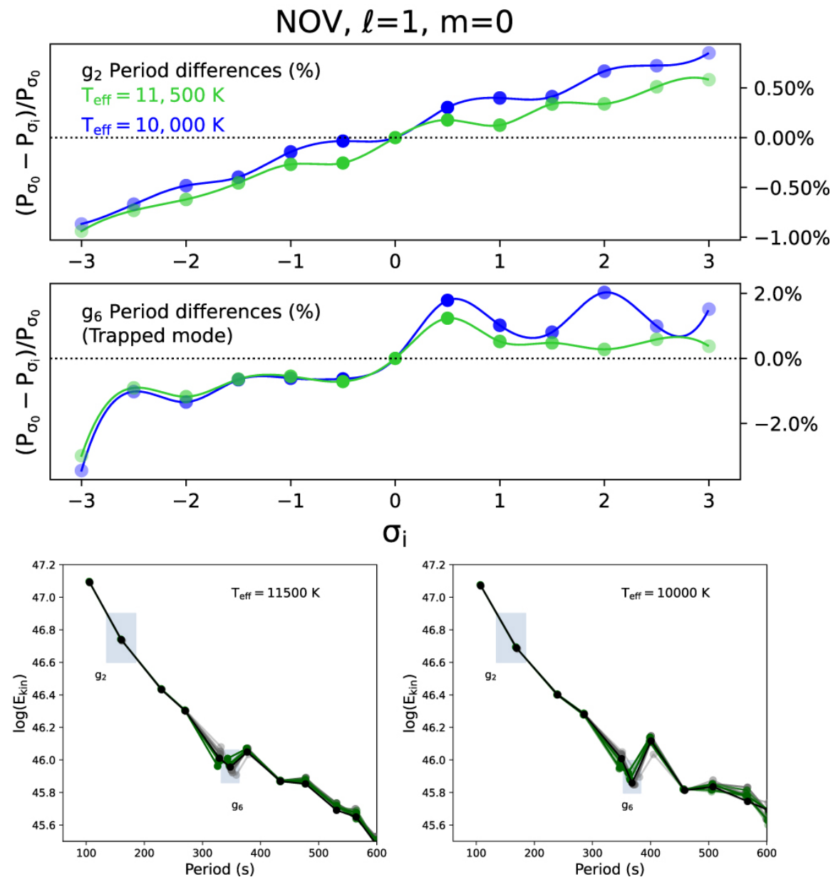
Figure 4. from Morgan T. Chidester et al 2023 Astrophys. J. 954 doi:10.3847/1538-4357/ace620 https://dx.doi.org/10.3847/1538-4357/ace620 © 2023. The Author(s). Published by the American Astronomical Society.
