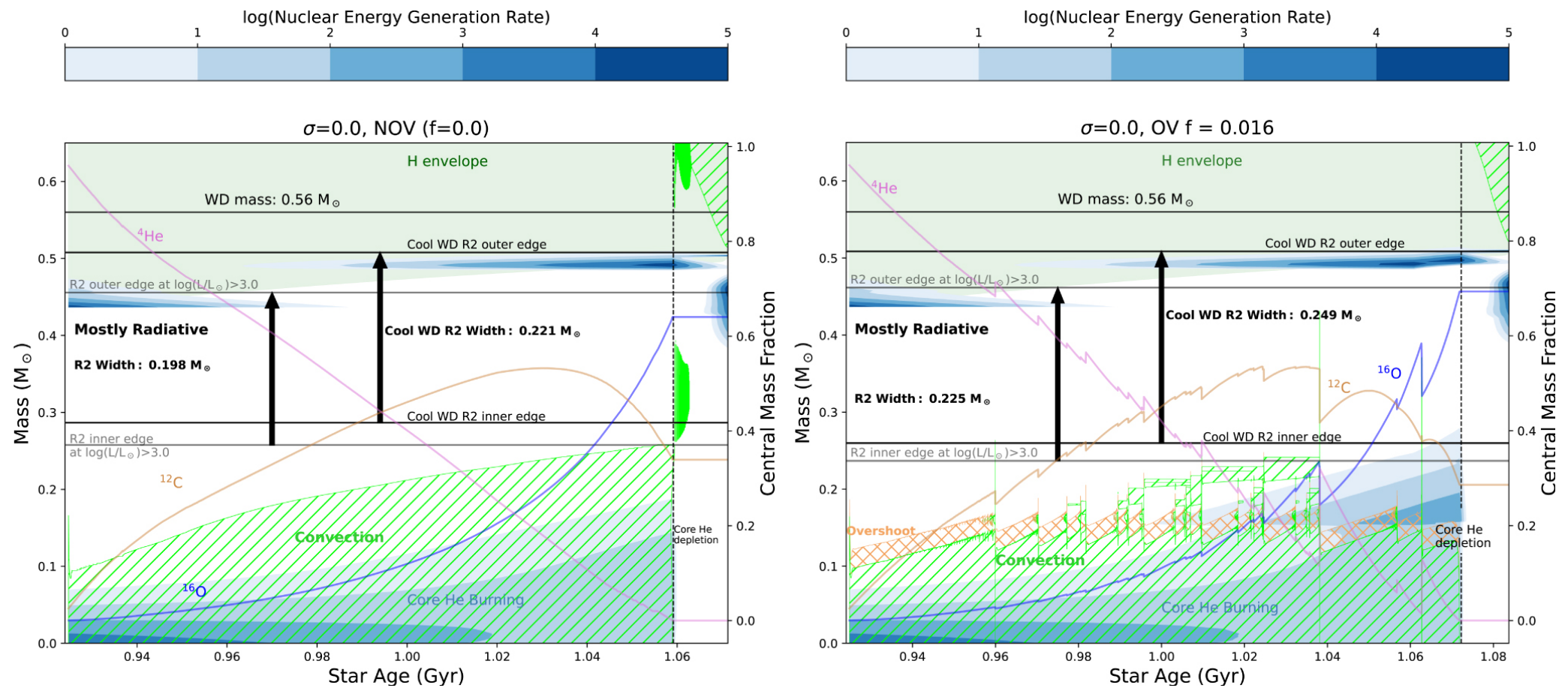
Figure 3. from Morgan T. Chidester et al 2023 Astrophys. J. 954 doi:10.3847/1538-4357/ace620 https://dx.doi.org/10.3847/1538-4357/ace620 © 2023. The Author(s). Published by the American Astronomical Society.
