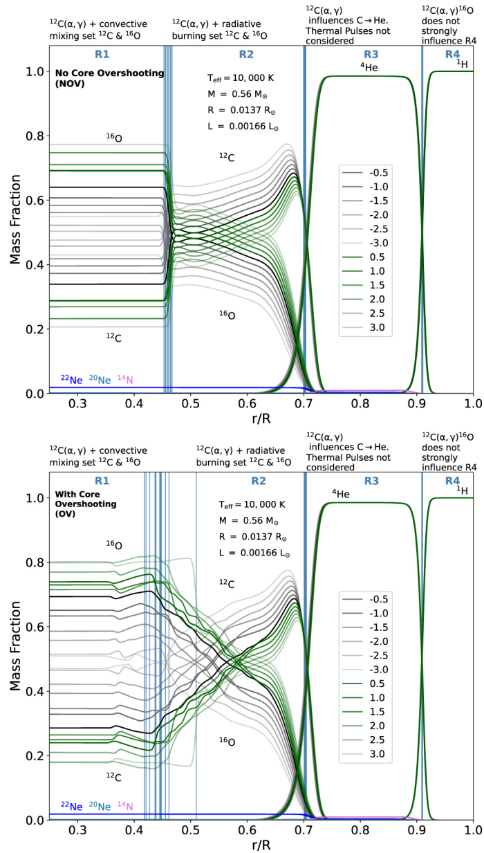
Figure 2. from Morgan T. Chidester et al 2023 Astrophys. J. 954 doi:10.3847/1538-4357/ace620 https://dx.doi.org/10.3847/1538-4357/ace620 © 2023. The Author(s). Published by the American Astronomical Society.
