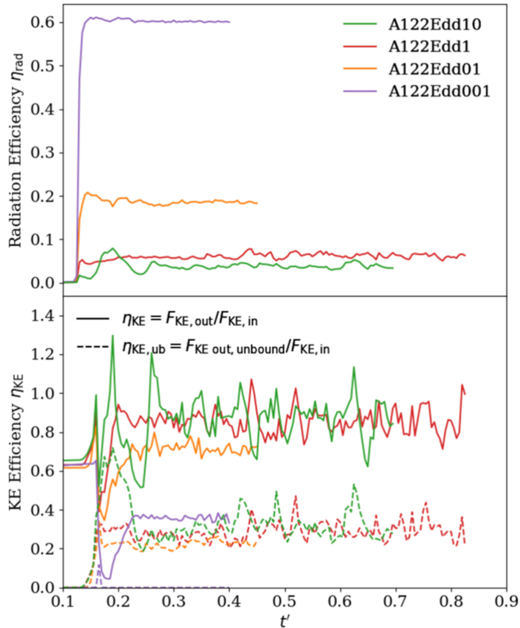
Figure 9. from Xiaoshan Huang et al 2023 Astrophys. J. 953 doi:10.3847/1538-4357/ace0be https://dx.doi.org/10.3847/1538-4357/ace0be © 2023. The Author(s). Published by the American Astronomical Society.
