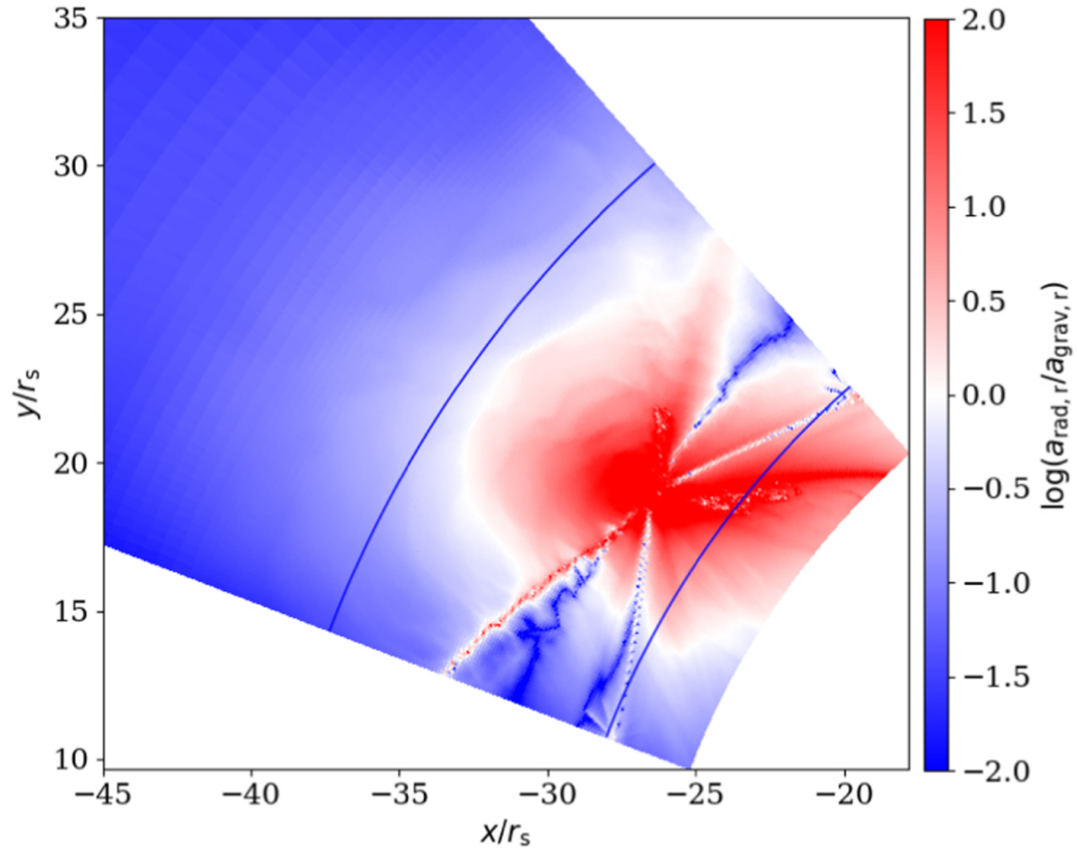
Figure 7. from Xiaoshan Huang et al 2023 Astrophys. J. 953 doi:10.3847/1538-4357/ace0be https://dx.doi.org/10.3847/1538-4357/ace0be © 2023. The Author(s). Published by the American Astronomical Society.
